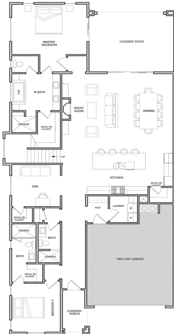
MAIN LEVEL FLOOR PLAN
